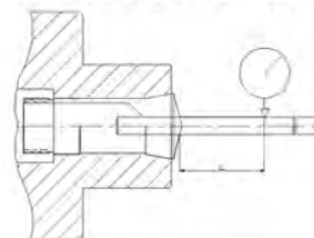
PULL-TYPE COLLETS
